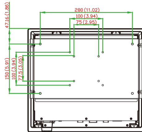
VESA Mounting Kit 4xM6 min. 10 mm, max. 12 mm deep mounting holes (280x150 mm) 8xM4 min. 10 mm, max. 12 mm deep mounting holes (100x100 mm/75x75 mm)
