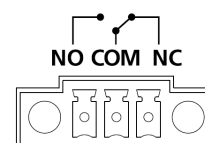
RELAY
